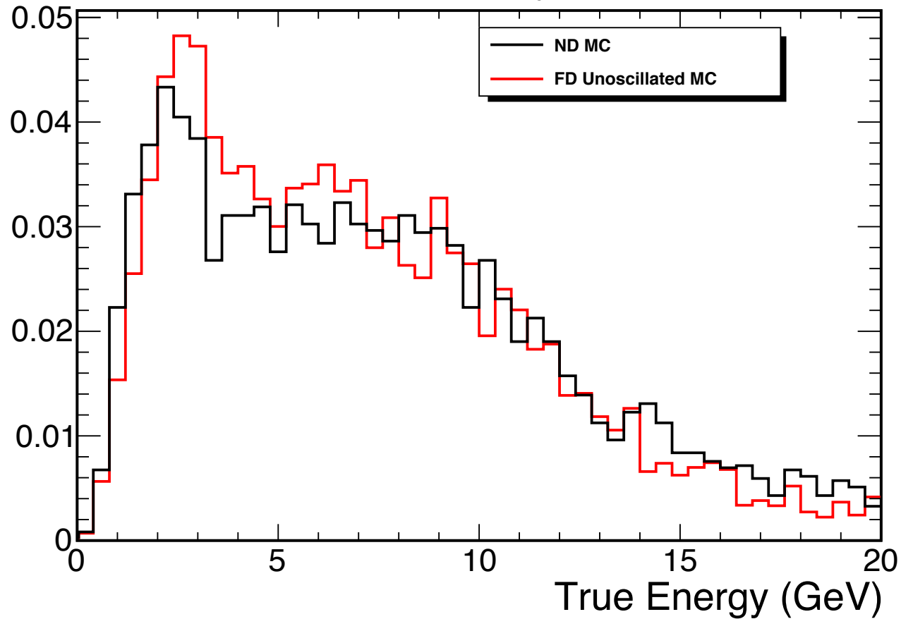
Area Normalized Beam \nu_e CC Event Rates
