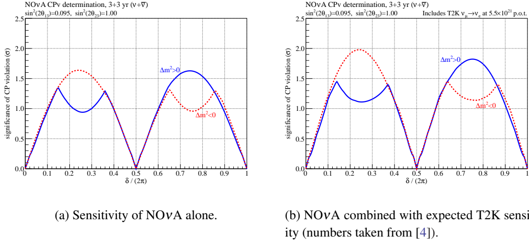
Figure 3: NOVA's sensitivity to CP violation ( \delta_{CP} \neq 0, \pi ) as a function of \delta_{CP} .
