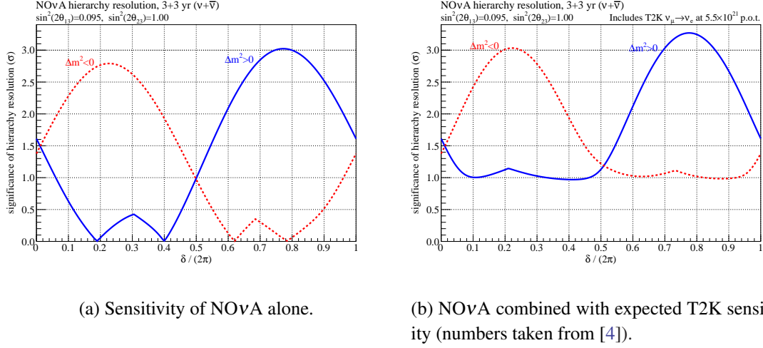
Figure 2: NOVA's sensitivity to the neutrino mass hierarchy as a function of \delta_{CP} .
