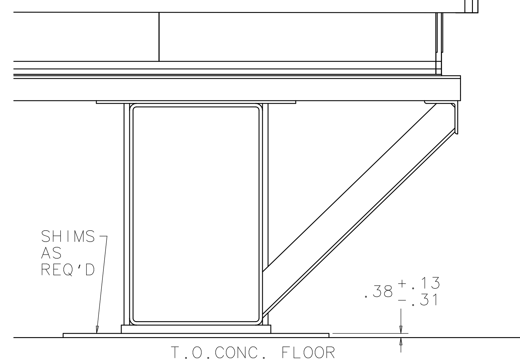
DETAIL A TYP. SHIMMING UNDER PALLET PAD SCALE: 1/16
