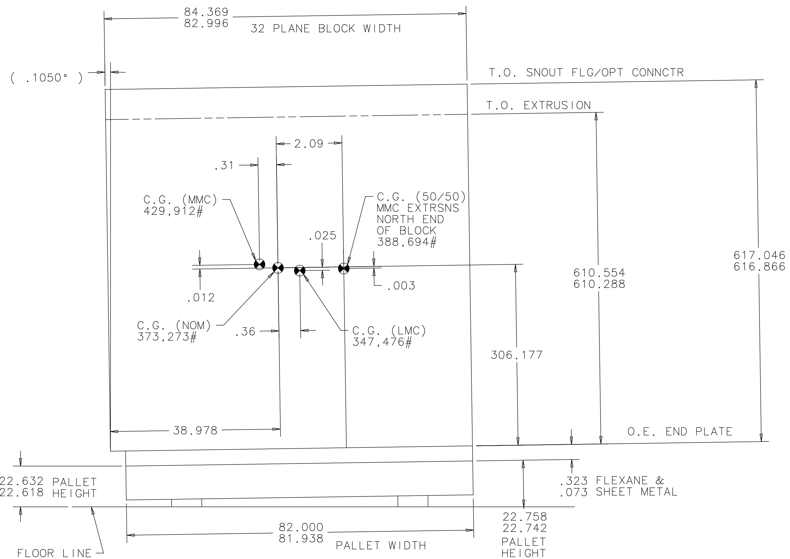
BLOCK ELEVATION SHOWN IN THE INSTALLED POSITION FOR TOP GUIDED INSTALLATION
